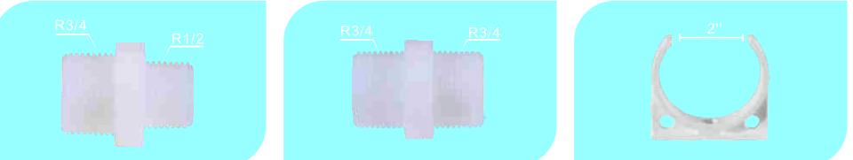
3/4外牙转1/2外牙直通M64 R3/4*R1/2 male connector M64 3/4外牙转3/4外牙直通M66 R3/4*R3/4 male connector M66 小单夹 small single clip XDJ
