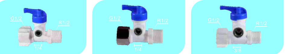
1/4管三通球阀带塑料螺帽1/4STQFM 1/4 tube three way plastic ball valve 1/4STQFM 1/4管三通球阀带不锈钢螺帽1/4STQFJM 1/4 tube three way stainless steel ball valve 1/4STQFJM 3/8管三通球阀带塑料螺帽3/8STQFM 3/8 tube three way plastic ball valve 3/8STQFM
