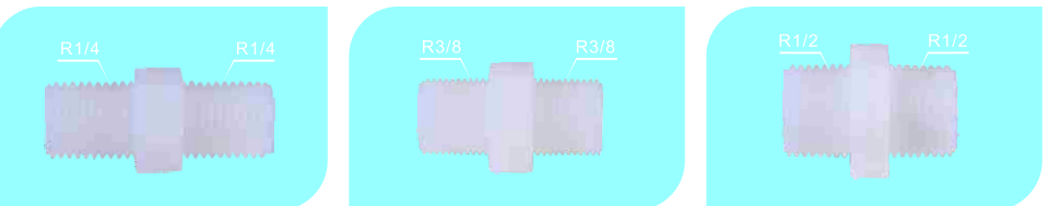
1/4外牙转1/4外牙直通M22 R1/4*R1/4 male connector M22 3/8外牙转3/8外牙直通M33 R3/8 *R3/8 male connector M33 1/2外牙转1/2外牙直通M44 R1/2*R1/2 male connector M44
